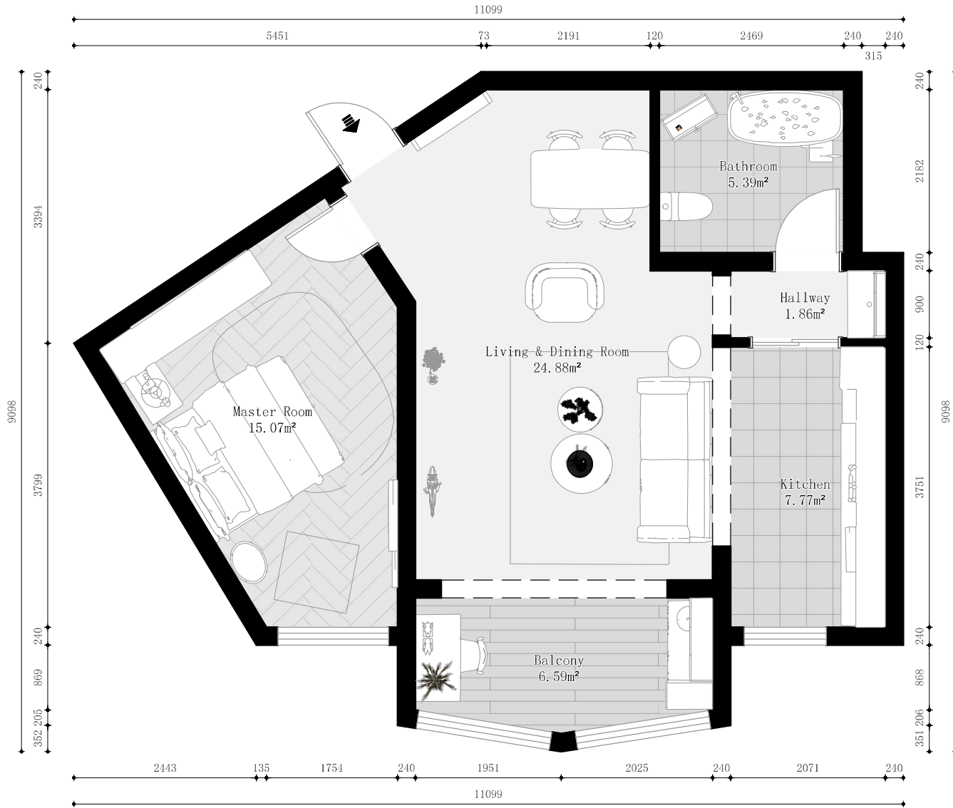
Full House Plan 1:70
