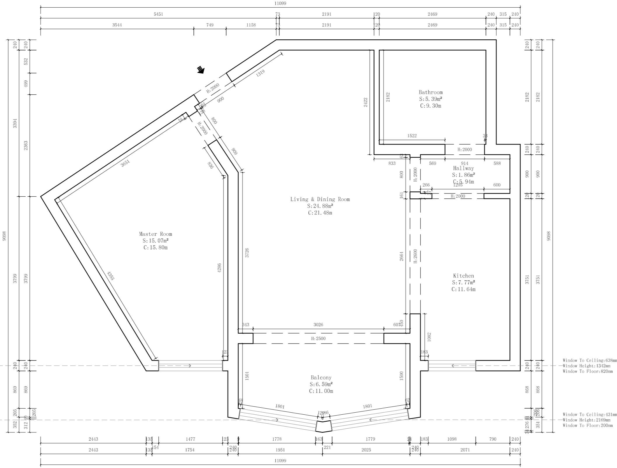
Floor Plan 1:50
